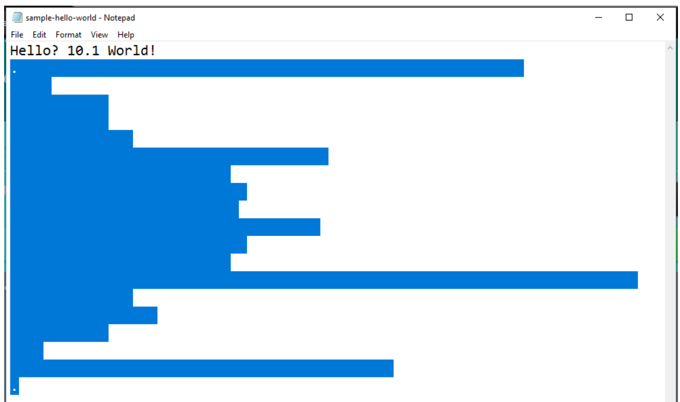
Figure 24.6: Sample Ghost-Message for “Hello? 10.1 World!” with both literal original message and highlighted invisible [dotted] ghost message
