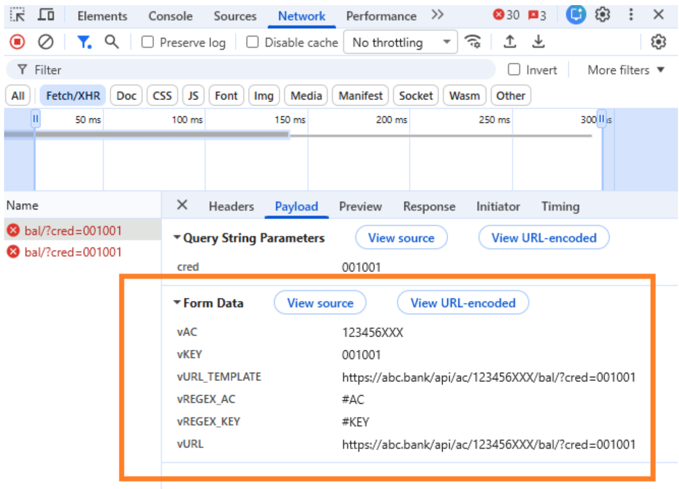
Figure 29.1: Under-the-hood debugging of HTTP POST payloads from Example 1
