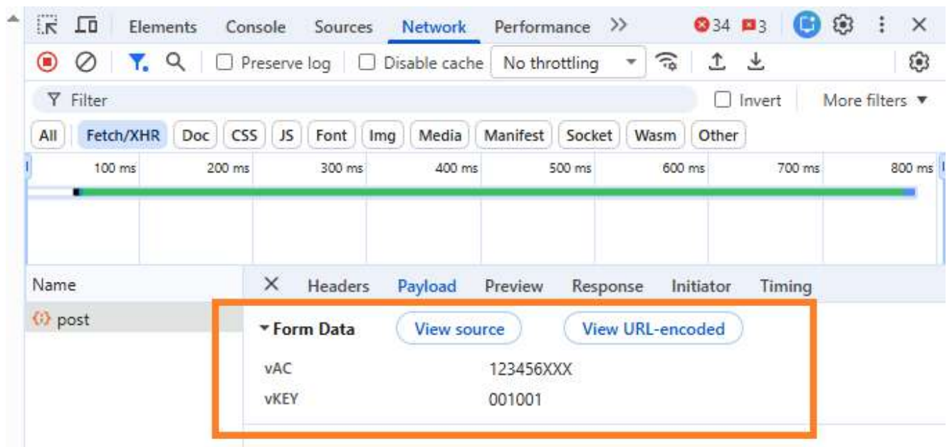
Figure 29.2: Under-the-hood debugging of HTTP POST payloads from Example 2
