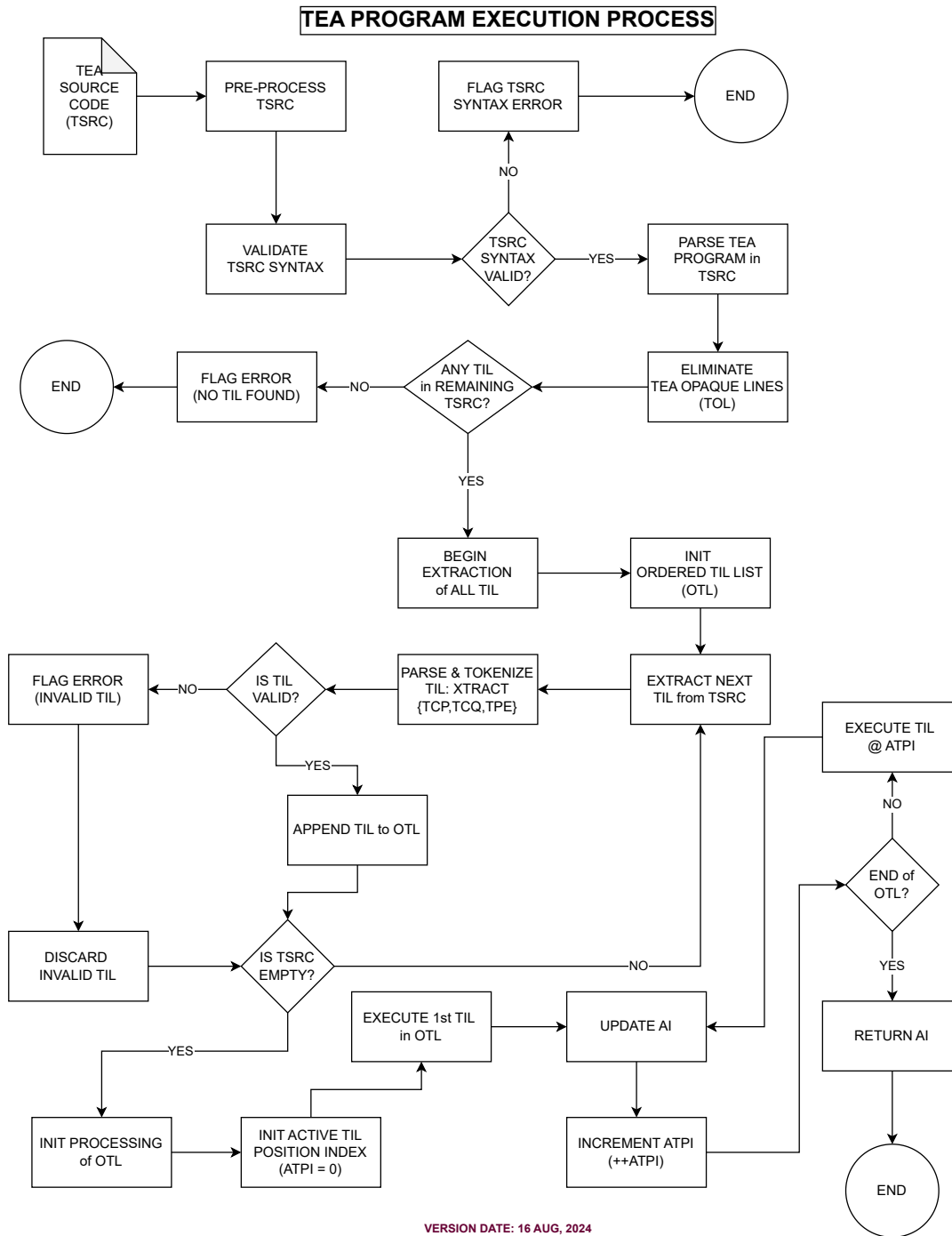
Figure 2.7: The TEA Program Execution Process.
