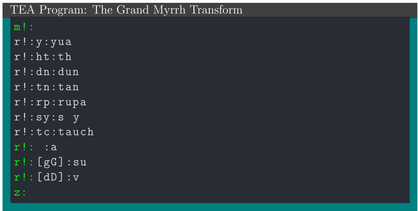
Figure 19.1: The Grand Myrrh Transform
